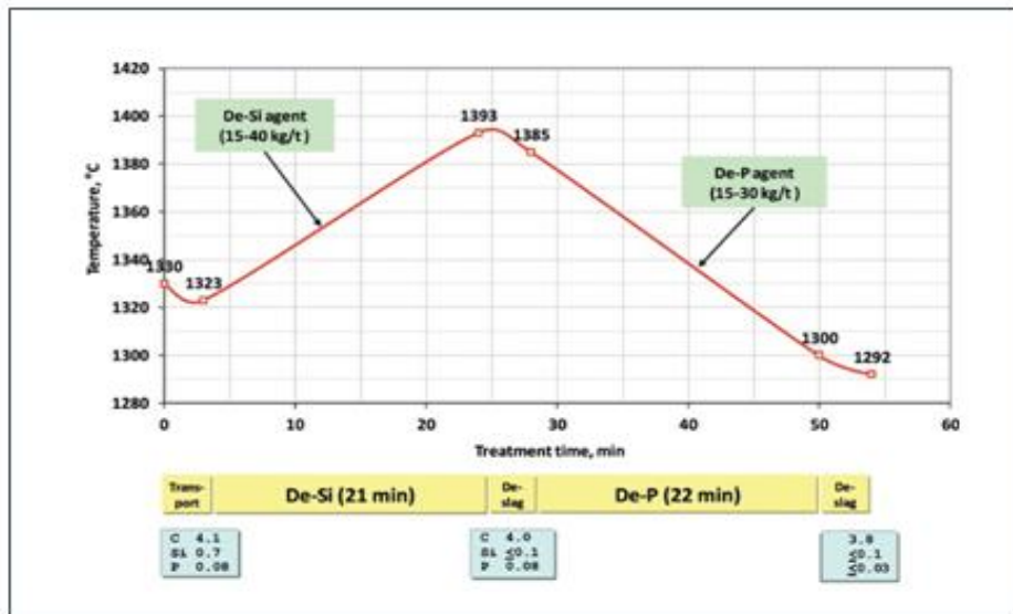
Principle of the compensation of temperature losses by Küttner process
