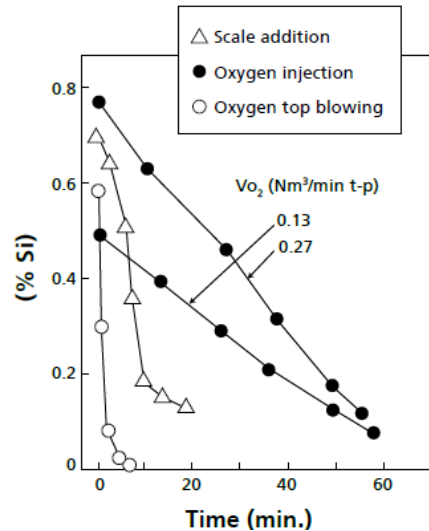
Comparison of desiliconization behavior
