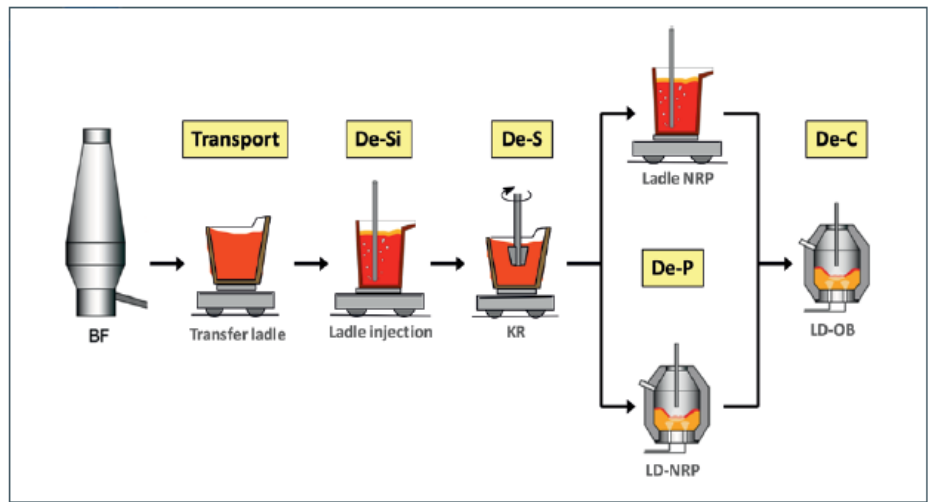
Zero slag process (ZSP) at NKK's Fukuyama works [10]
