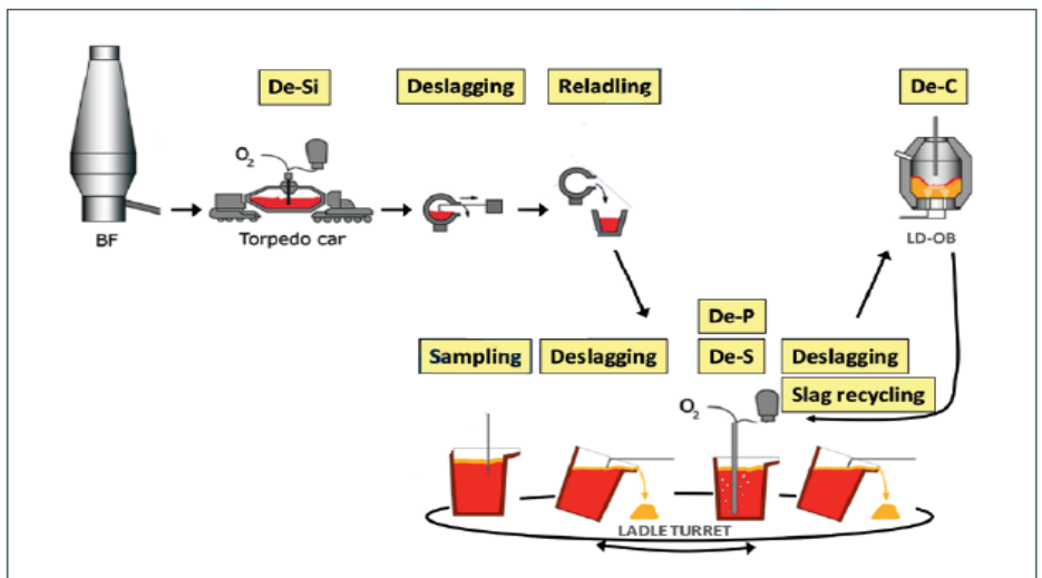
Ladle – based hot pretreatment process at Nippon Steel, Oita works [9]
