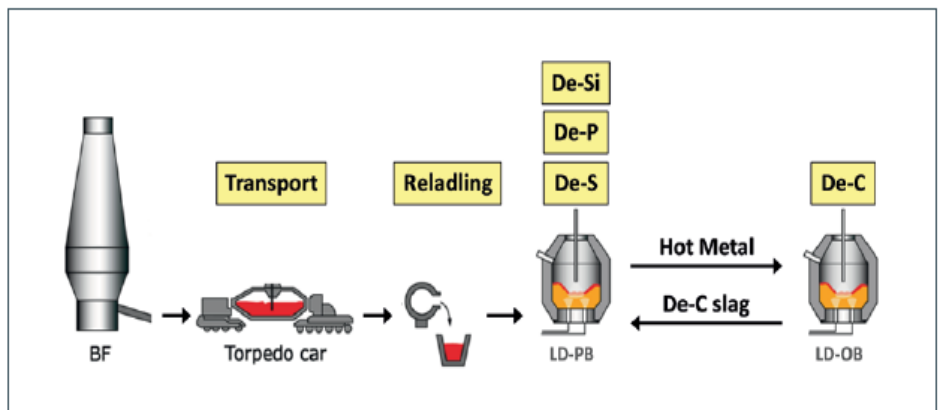
Converter – based pretreatment process LD – ORP at Nippon Steel, Nagoya works [9]
