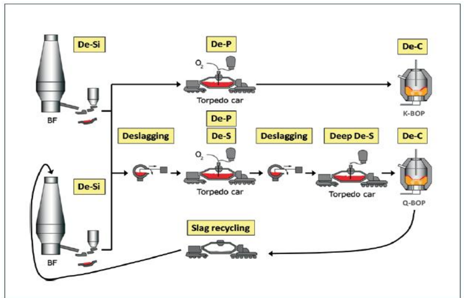
Hot metal pretreatment process at Kawasaki Steel, Chiba works [8]
