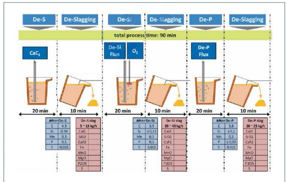
Alternative sequence of hot metal pretreatment within produce within the conventional BF-BOF route
