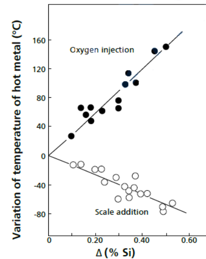
Desiliconization with gaseous and solid oxygen and variation of the hot metal temperature for desiliconization [5]
