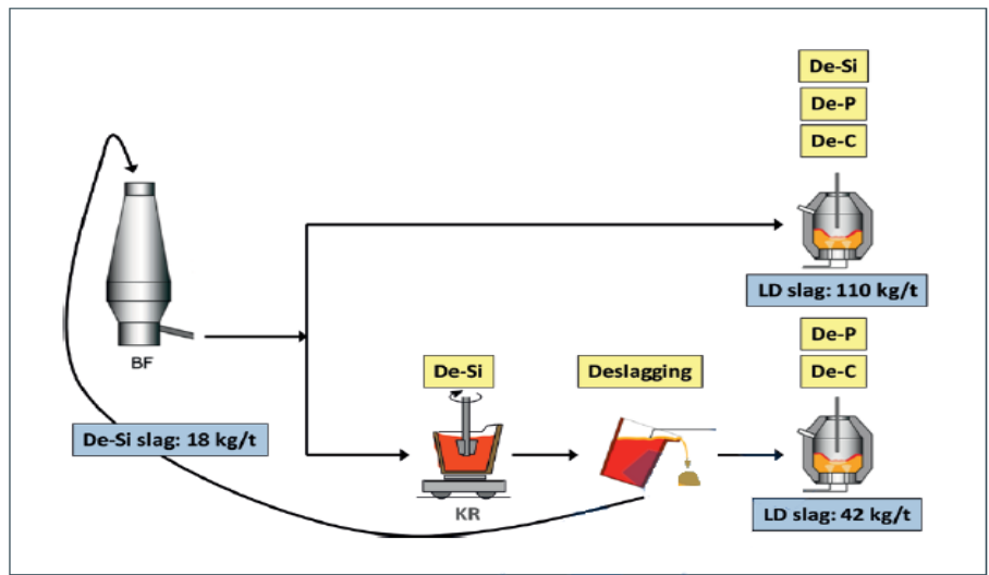
Process flow scheme of Nippon Steel's slag minimum refining process (SMP) [7]
